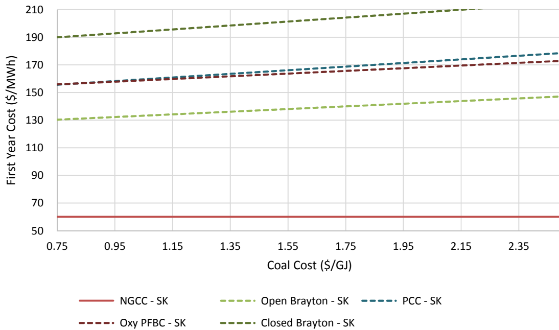
Figure 9: First Year Cost of Power vs Coal Cost
